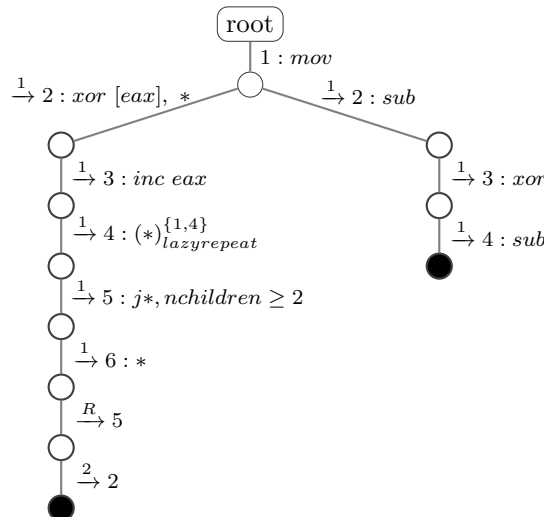
Figure 6: Traversal tree with xor loop pattern (Figure 5) and mov->sub->xor->sub
