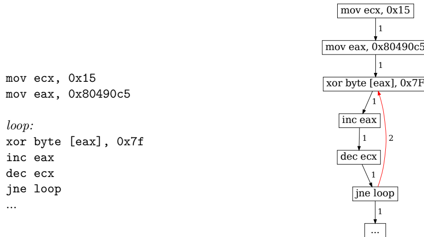
Figure 1: xor decryption loop and its CFG
