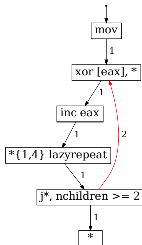
Figure 5: Pattern and its traversal
