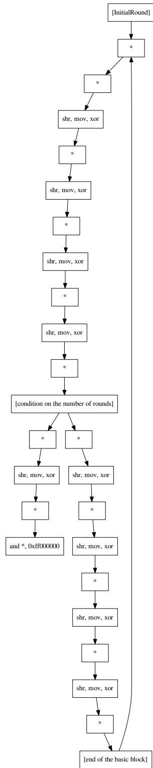
Figure 7: A simplified graphical representation of a pattern that allows the detection of an AES implementation. The general structure of the algorithm is preserved.
